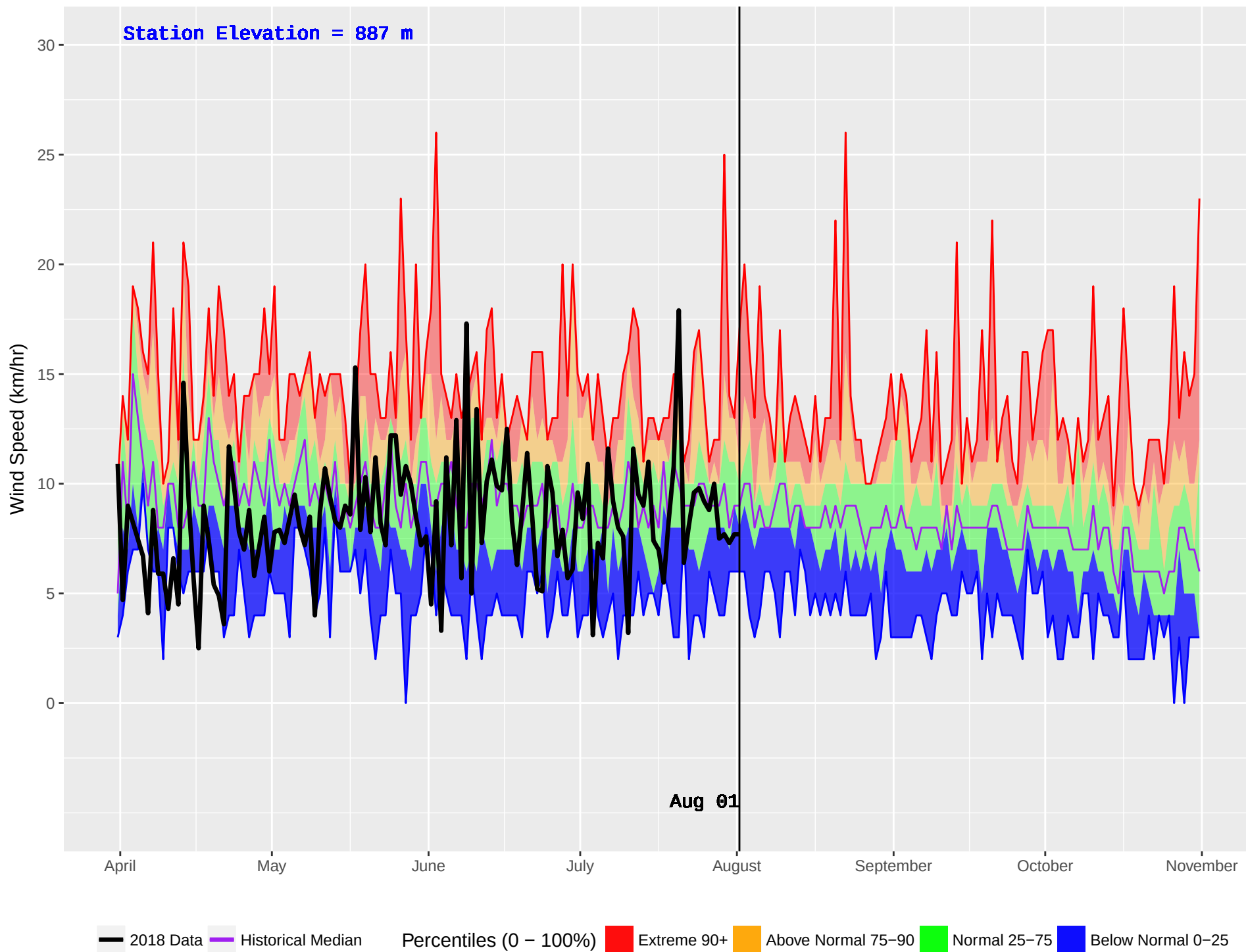
CRAWFORD (873) : Historical (2004–2016) and Current (2018) Daily Wind Speed
