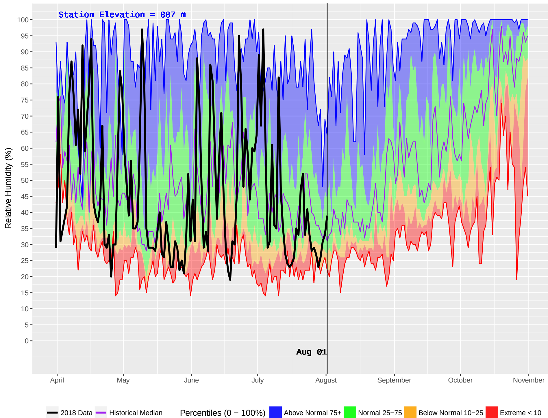
CRAWFORD (873) : Historical (2004–2016) and Current (2018) Daily Relative Humidity
