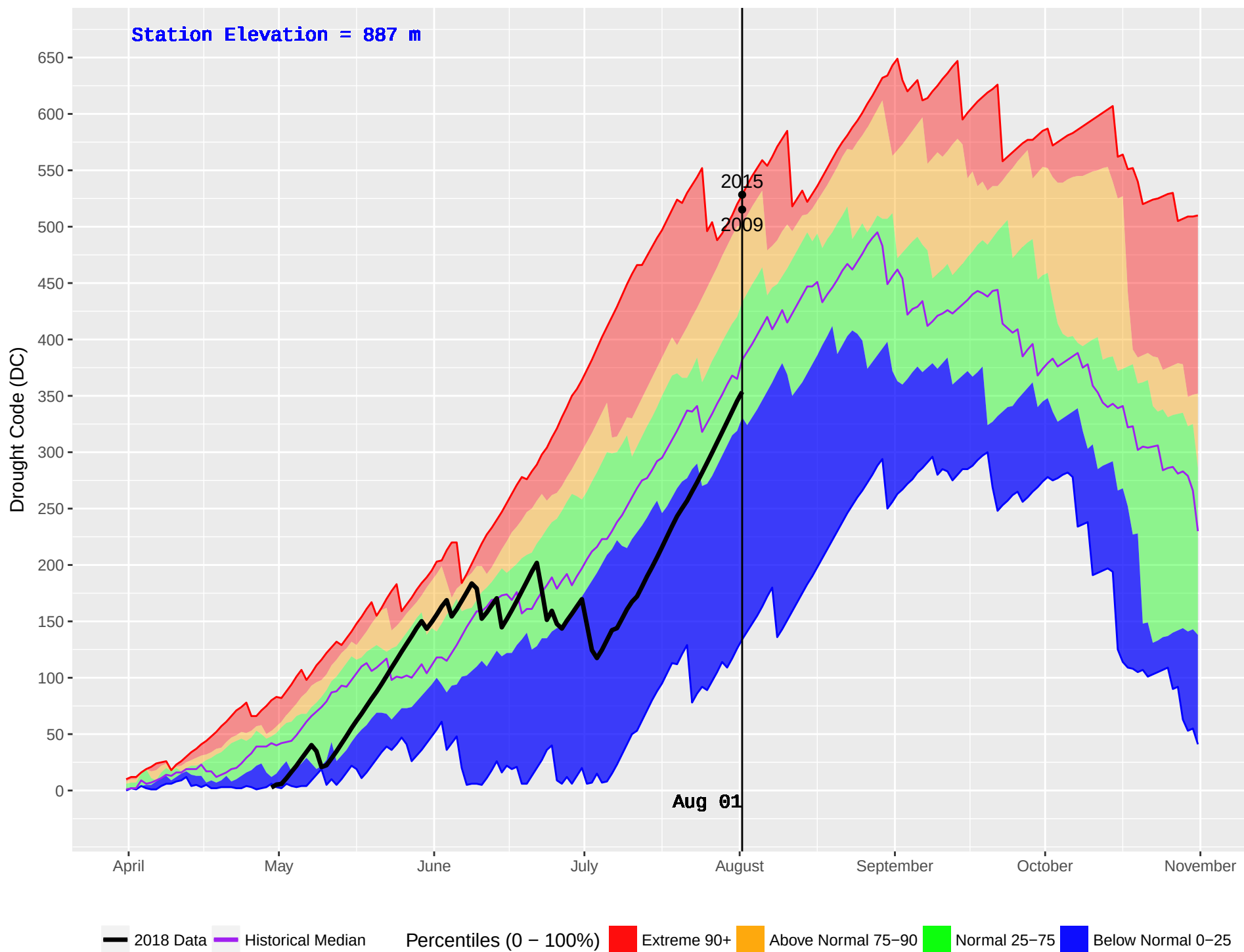
CRAWFORD (873) : Historical (2004–2016) and Current (2018) Daily Drought Code (DC)
